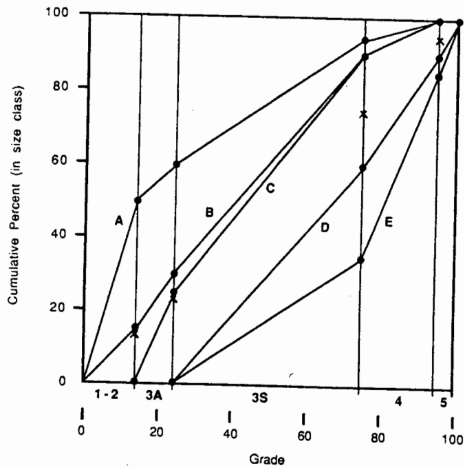
Figure 6 FIVE CUMULATIVE DISTRIBUTIONS OF ORDERED-CATEGORY DATA. The upper panel shows a conventional display, using shading to represent the ordered variable, which is intensity of abnormality. The lower panel shows the same information cast in cumulative form. Source: Ref. (13).
