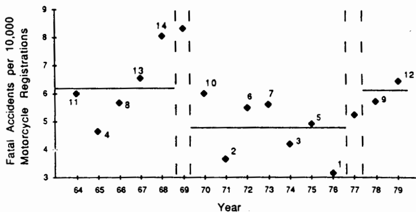
Figure 11 FATAL MOTORCYCLE ACCIDENTS IN COLORADO WITH AND WITHOUT A HELMET LAW. Numbers appearing near the data points are ranks (1 is smallest, 14 is largest) of the observations. Horizontal lines are simple averages of the rates for the period. The ranks justify the conclusion that the lower rate during the helmet law era is not likely to be a chance aberration. The data are the same as in Table 3. Source: Ref. (12).
