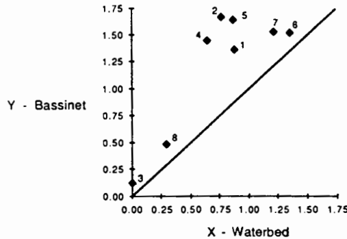
Figure 12 APNEA IN EIGHT PREMATURE INFANTS UNDER TWO SLEEP CONDITIONS. The numerical values represent number of episodes of apnea (exceeding 20 seconds) per hour of sleep on a waterbed (W) or bassinet (B). These are the data of Table 4. Source: Ref. (11).
