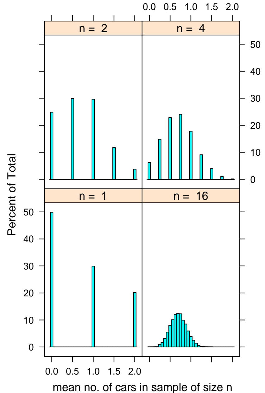
Figure 1: Illustration of Central Limit Theorem
